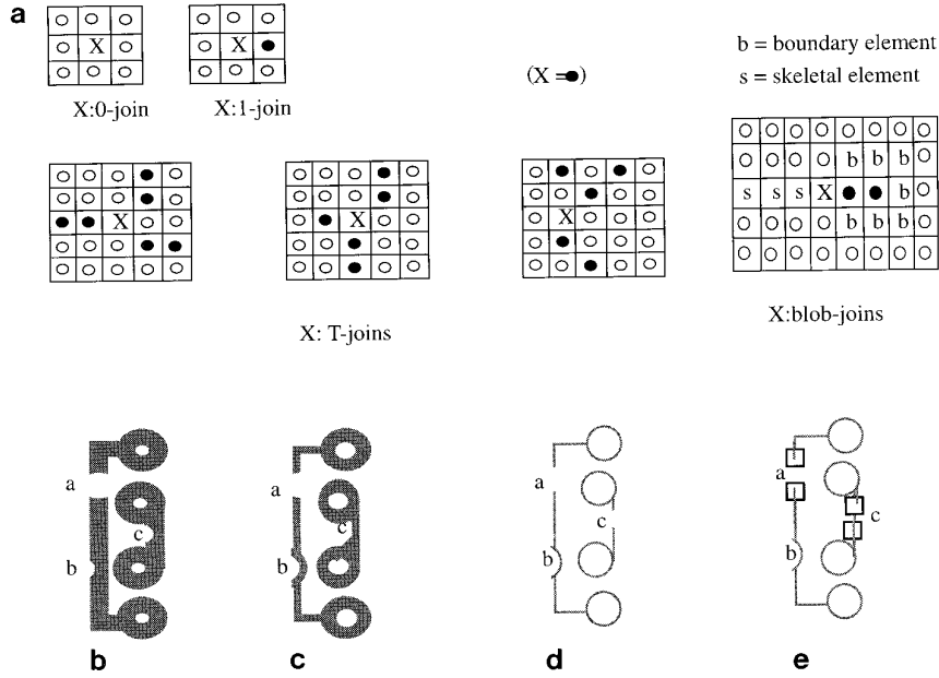
FIG. 14. Verification of minimum trace width. (a) n -joins, T-joints, and blob-joints; (b) defect image; (c) after contracting n times; (d) after thinning m times; and (e) with joints identified.
