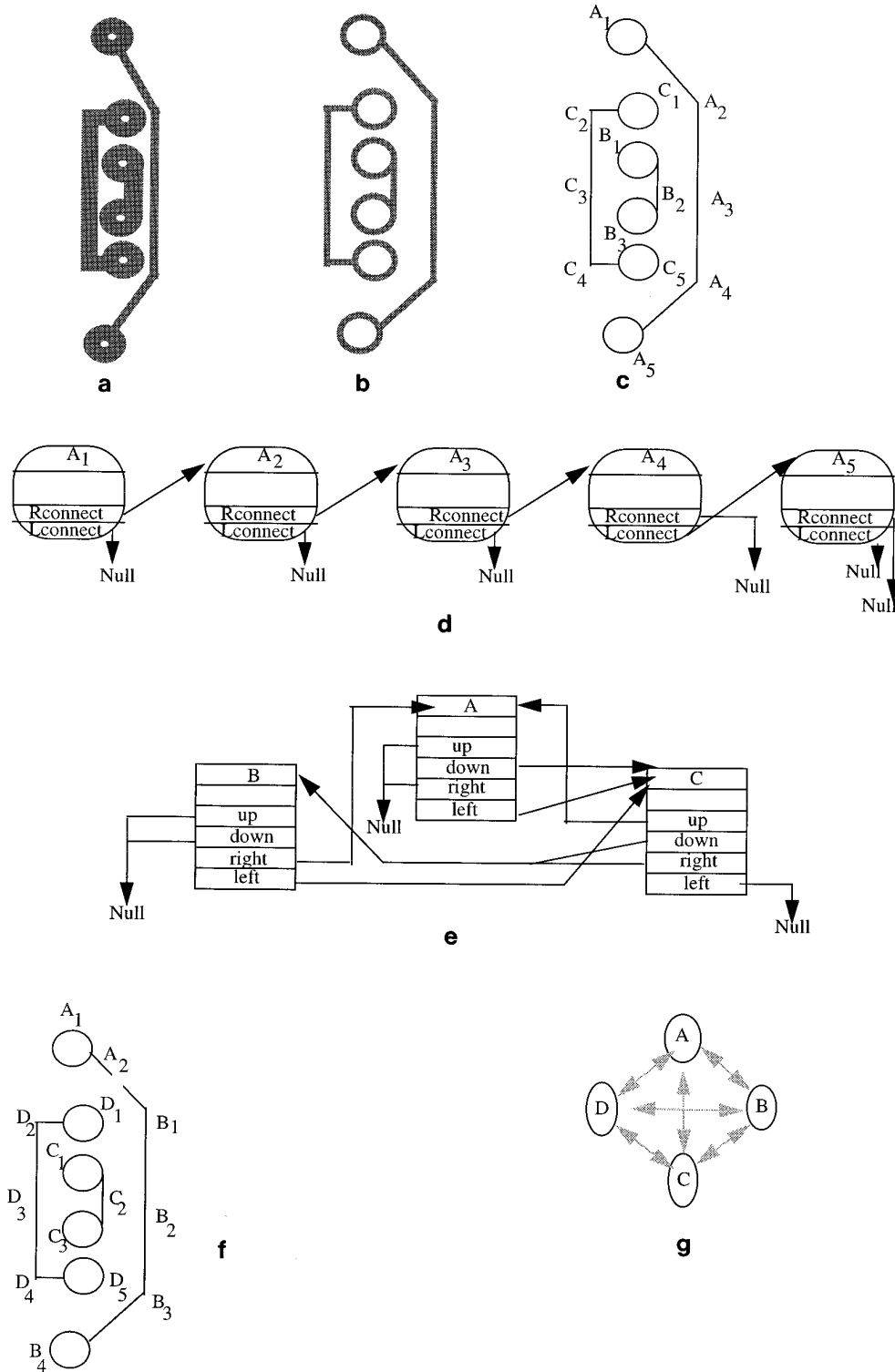
FIG. 8. Graph matching using pattern attributed hypergraph. (a) PCB subimage pattern, (b) thinned PCB pattern, (c) pruned PCB pattern with labels, (d) representation of RAG for segment A in (c), (e) graphical representation of PAHG for the subimage pattern (a), (f) pruned defective PCB pattern with labels, and (g) PAHG for (f).
